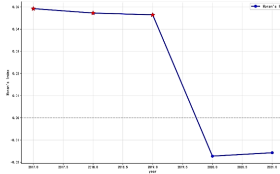
Fig. 1. Temporal evolution of the global Moran's I for CO 2 emission intensity.
